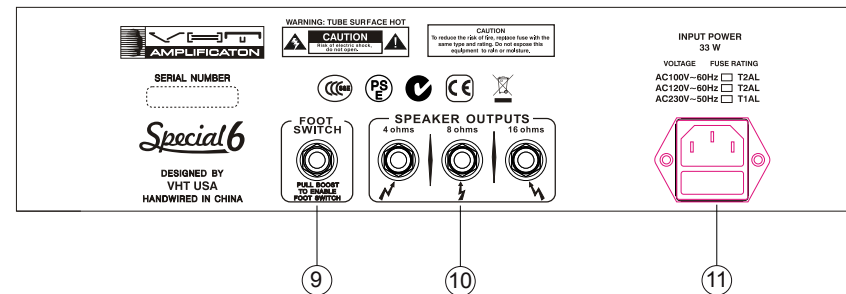
Fig. 2: The Rear Panel
